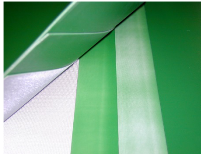
3-layered Stepped Splice
