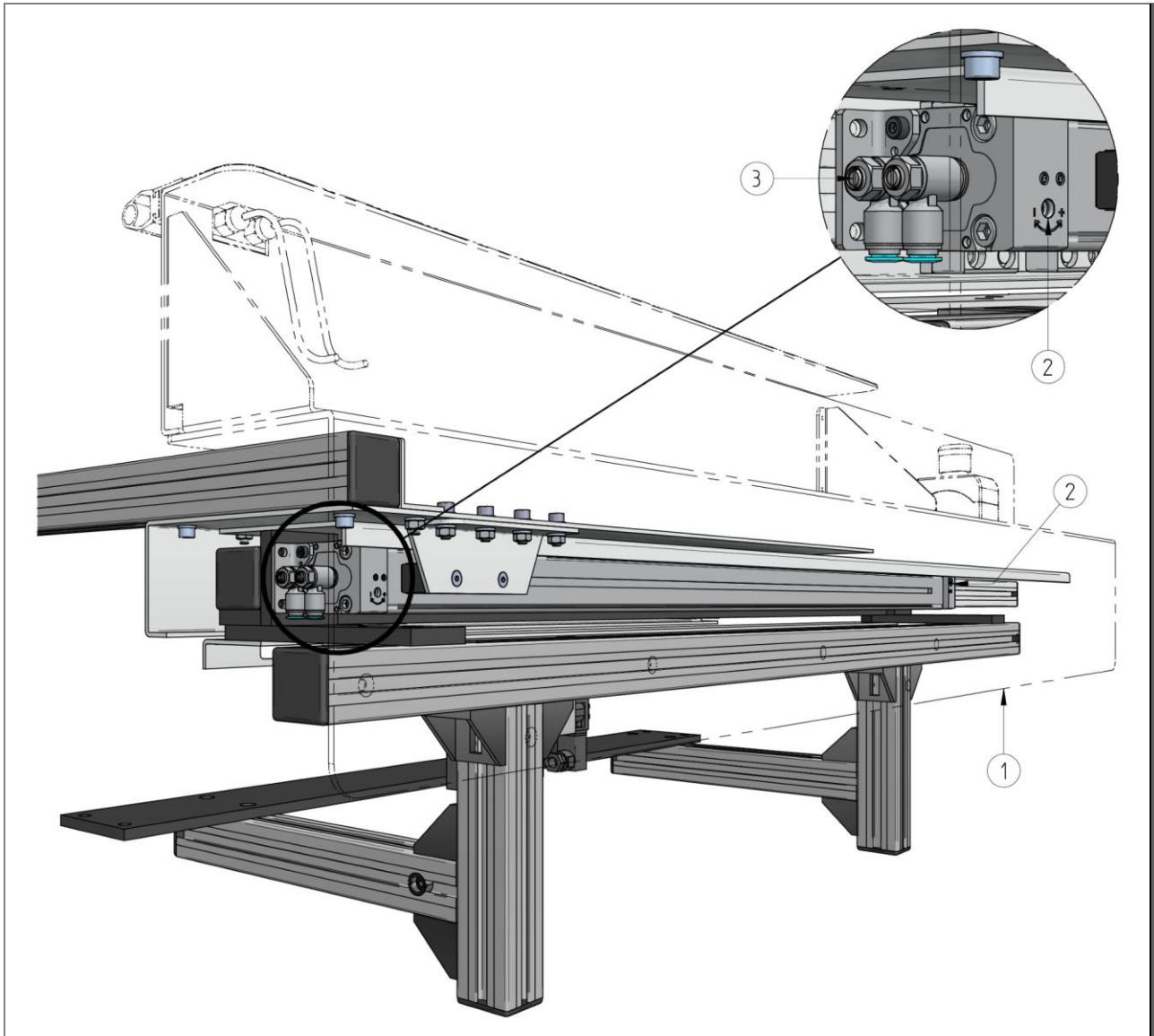
Fig. 9: Access points (maintenance tasks)
