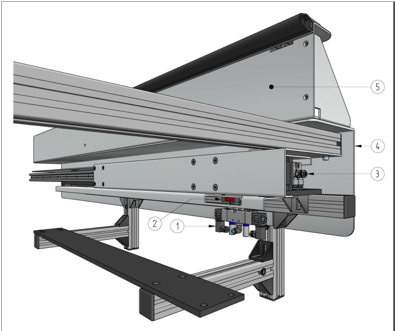
Fig. 4: General view from the front
